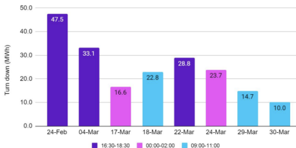
MWh reduction per event by date
