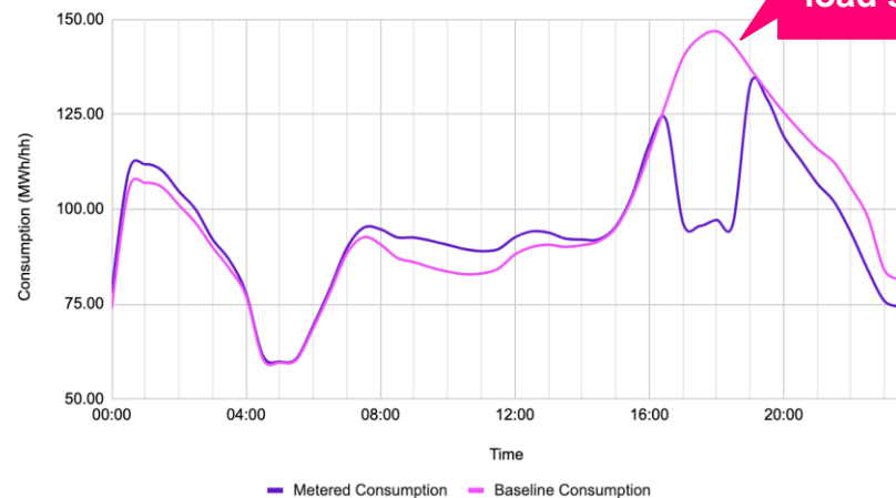
Consumption Profile for Session 5 (17:00-19:00)
